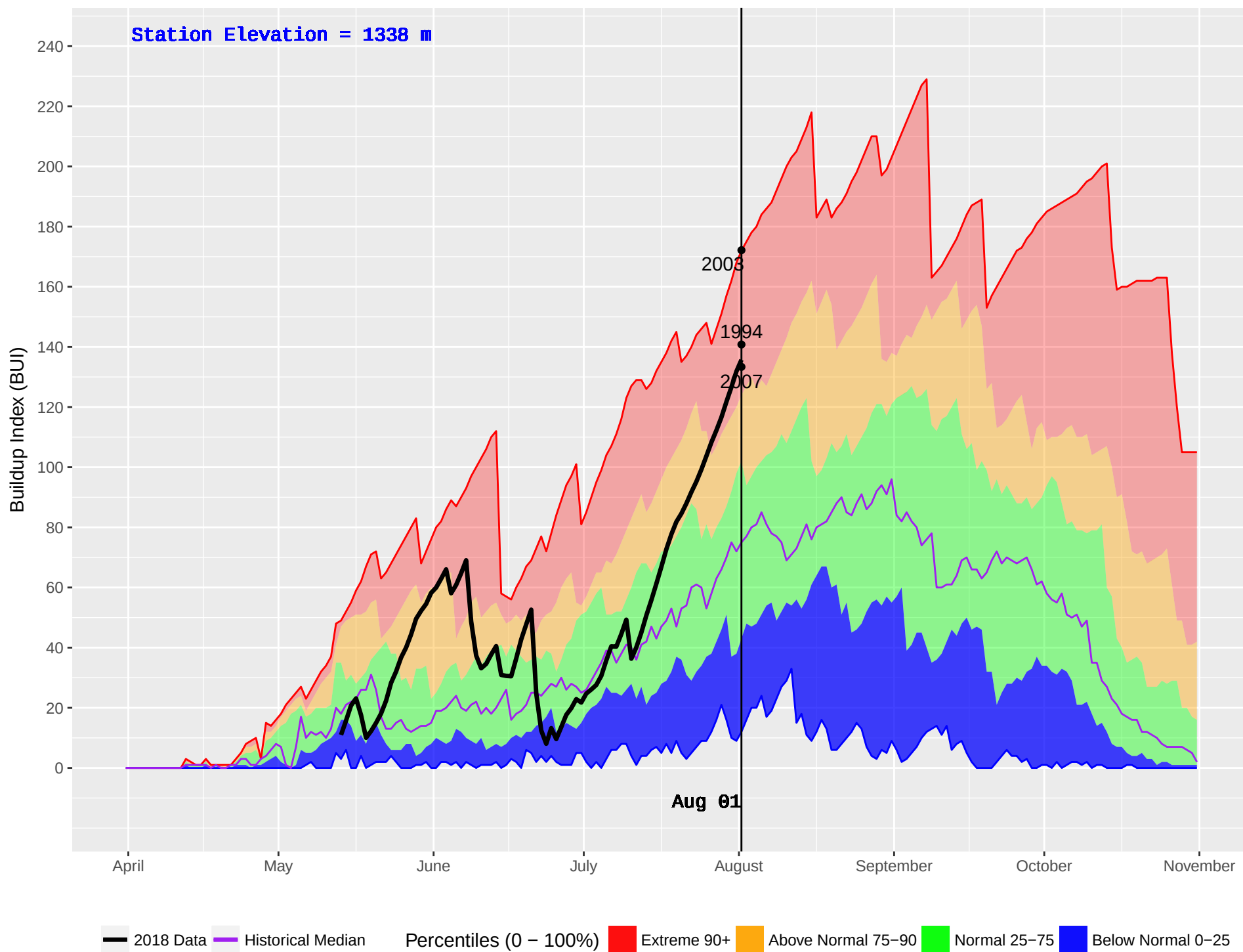
EIGHT MILE (391) : Historical (1980–2016) and Current (2018) Daily Buildup Index (BUI)
