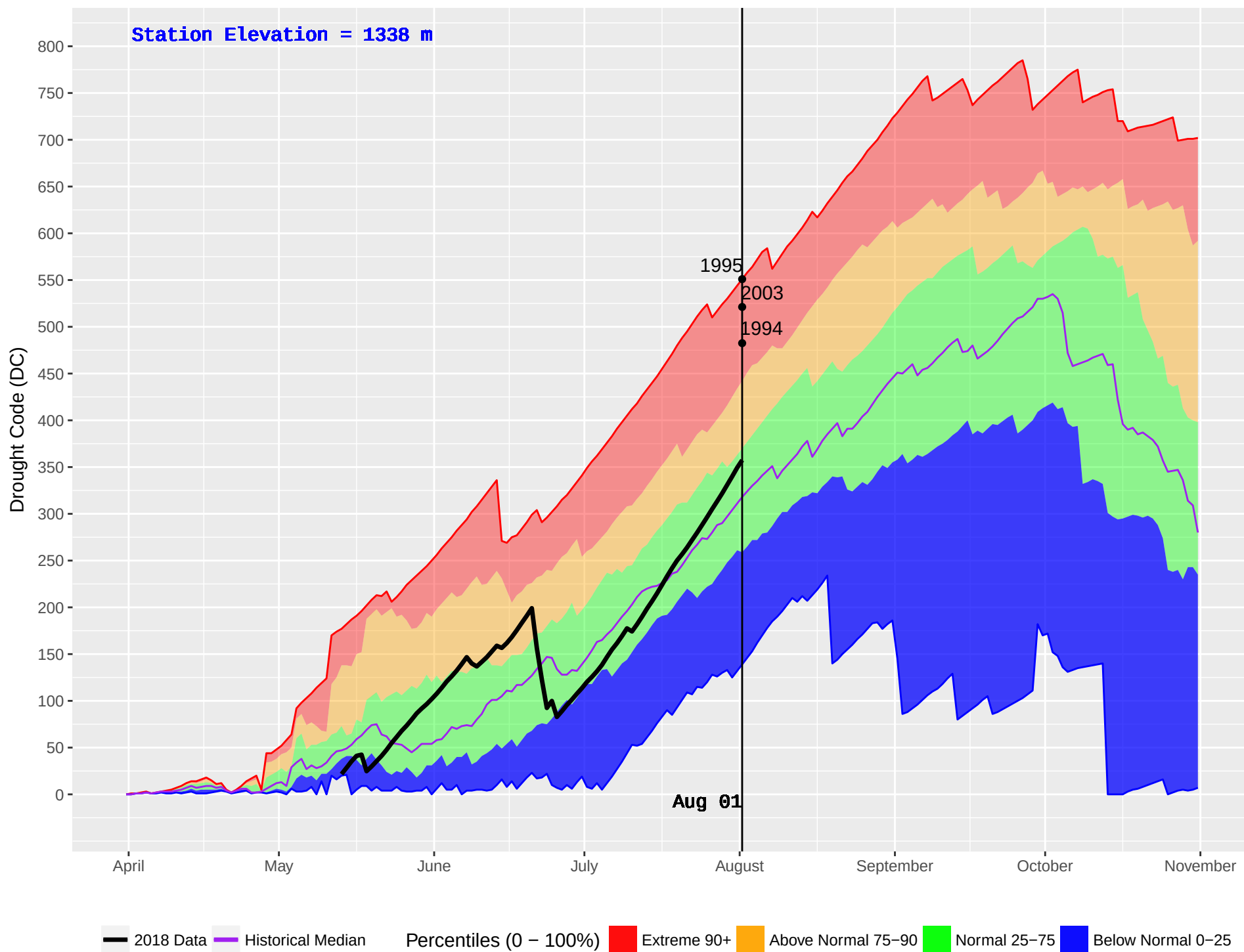
EIGHT MILE (391) : Historical (1980–2016) and Current (2018) Daily Drought Code (DC)
