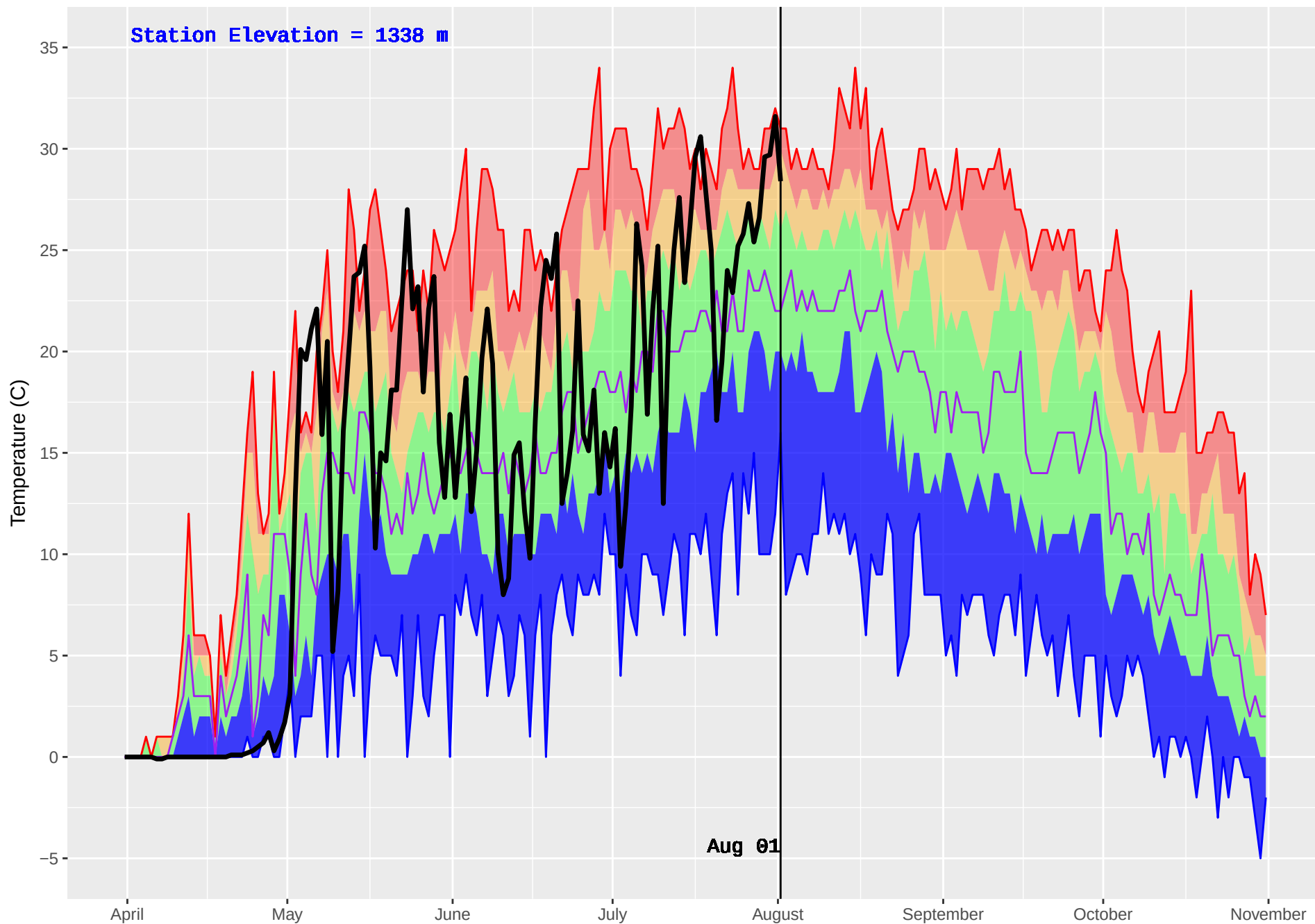
EIGHT MILE (391) : Historical (1980–2016) and Current (2018) Daily Temperature
