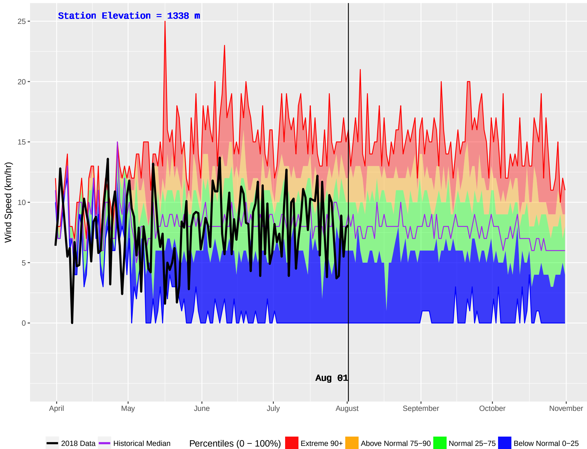
EIGHT MILE (391) : Historical (1980–2016) and Current (2018) Daily Wind Speed
